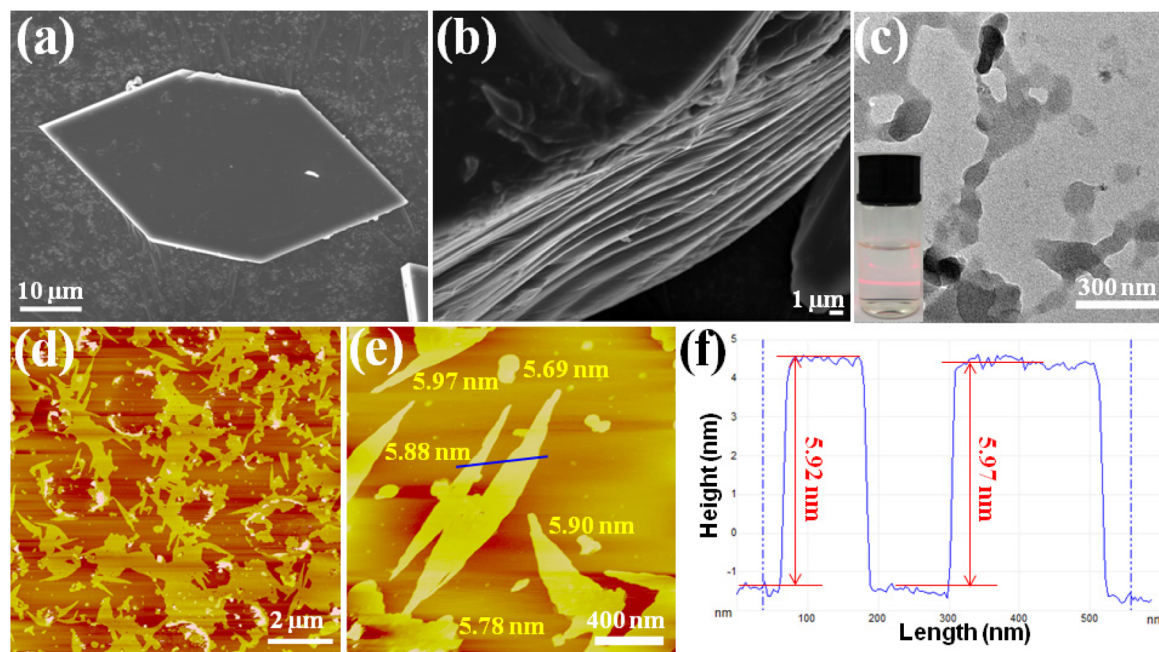
Fig. 2 (a) SEM image of the hexagonal Cu-MOF. (b) SEM image of the cross-section of the Cu-MOF. (c) TEM image of Cu-MOF nanosheets; inset: photograph of the Tyndall effect of Cu-MOF nanosheet suspension. (d and e) AFM images of Cu-MOF nanosheets. (f) Height profile, color-coded blue, is measured along the corresponding track shown in (e).
