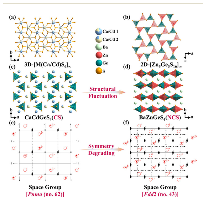
Fig. 2 Structural difference in \text{CaCdGeS}_4 and \text{BaZnGeS}_4 . (a) The formed 6-coordinated [\text{Ca/CdS}_6] octahedra in \text{CaCdGeS}_4 ; (b) the formed 4-coordinated [\text{ZnS}_4] tetrahedra in \text{BaZnGeS}_4 ; (c and d) the crystal structures of \text{CaCdGeS}_4 and \text{BaZnGeS}_4 viewed along the c direction; (e and f) detailed spatial symmetry operations in \text{CaCdGeS}_4 ( Pnma ) and \text{BaZnGeS}_4 ( Fdd2 ).
