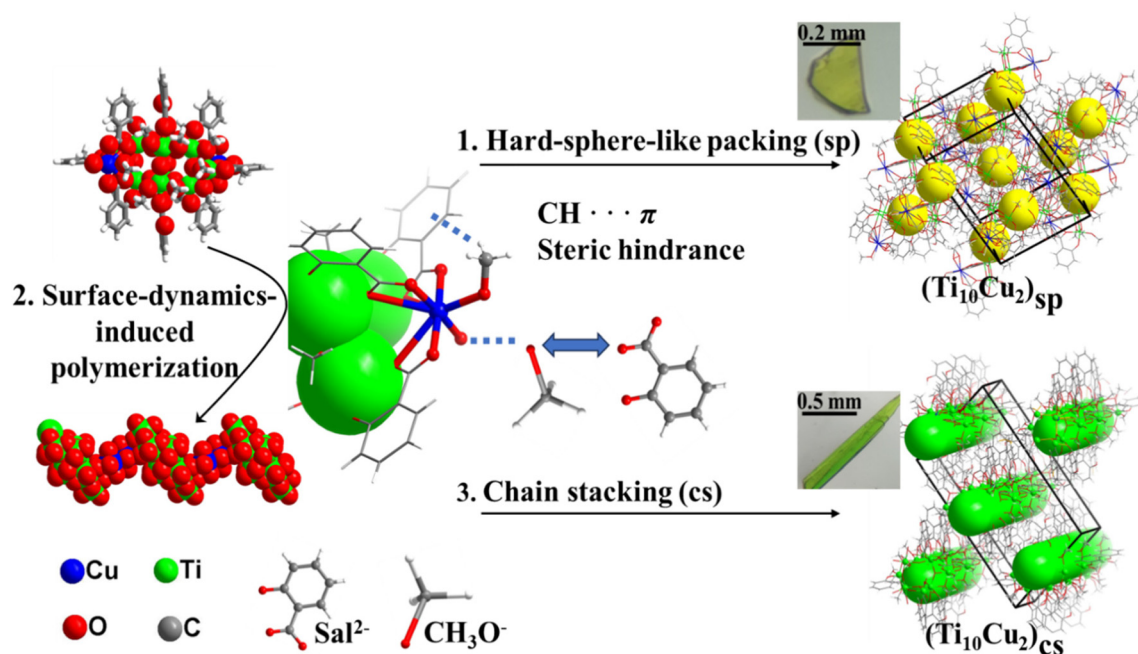
Fig. 1 Schematic illustration of the crystallization of {Ti 10 Cu 2 } into either hexagonal superlattices and block crystals (top) or, in the absence of one terminal -OMe, rod-like supercrystals (bottom). The OMe-Cu fragments dynamically detached from {Ti 10 Cu 2 } clusters and Sal-Cu fragments are grafted to {Ti 10 Cu 2 } clusters to favour 1D alignment of the clusters.
