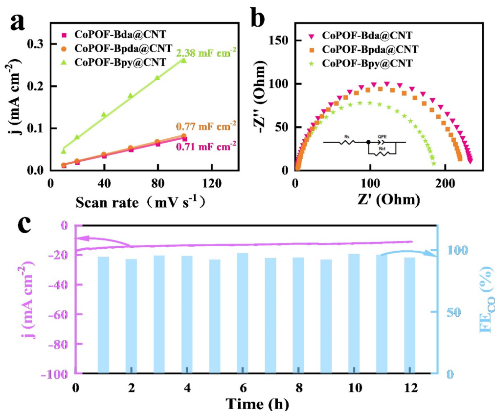
Fig. 4 (a) C_{dl} values of CoPOF-Bpy@CNT, CoPOF-Bda@CNT, and CoPOF-Bpda@CNT in the non-faradaic region with various scan rates ( 10\text{--}100 \text{ mV s}^{-1} ); (b) Nyquist plots by EIS; (c) measurements for assessing the long-term stability of CoPOF-Bpy@CNT at -0.7 \text{ V} vs. RHE in a \text{CO}_2 -saturated 0.5 \text{ M KHCO}_3 solution for 12 h.
