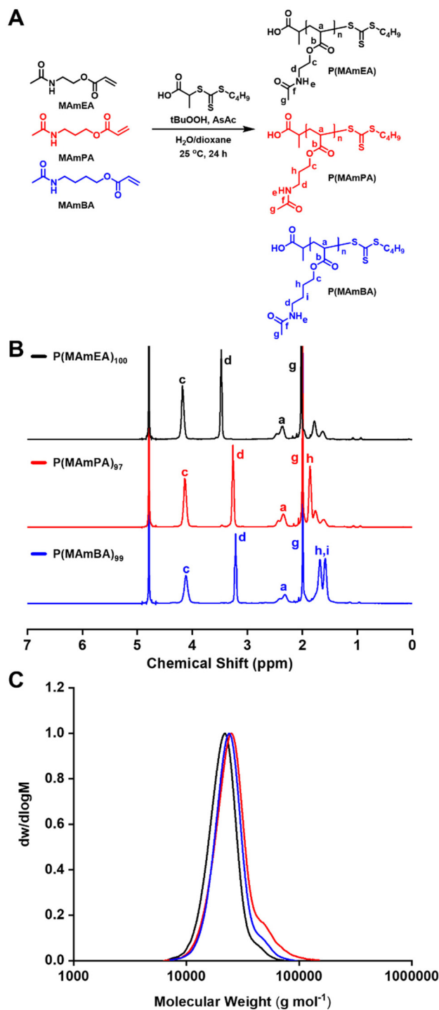
Fig. 2 (A) Synthesis pathway of homopolymers; (B) ^1\text{H} NMR spectra of P(MAmEA) 100 , P(MAmPA) 97 and P(MAmBA) 99 ; (C) SEC traces of P(MAmEA) 100 ( M_n = 20\,000 , D_M = 1.10 ), P(MAmPA) 97 ( M_n = 23\,900 , D_M = 1.17 ) and P(MAmBA) 99 ( M_n = 22\,700 , D_M = 1.12 ).
