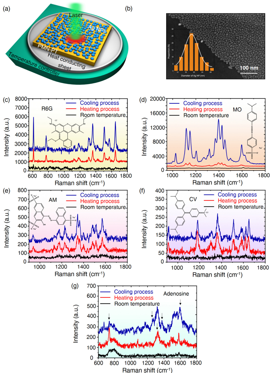
Fig. 3 (a) Schematic diagram of the SERS measurement experiment in the study. (b) SEM image of the prepared PMN-PT/Ag NP substrate and (inset) the corresponding histogram of particle size distribution. SERS spectra recorded at RT and variable temperature from 20 °C (100 °C) to 100 °C (20 °C) at a rate of 2.5 °C s -1 for (c) R6G (10 -7 M), (d) MO (10 -7 M), (e) AM (10 -7 M), (f) CV (10 -7 M), (g) adenosine (10 -3 M).
