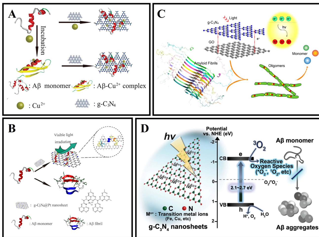
Fig. 5 (A) The ultrathin g\text{-C}_3\text{N}_4 nanosheets can effectively inhibit \text{Cu}^{2+} induced \text{A}\beta aggregation and disaggregate the preformed \text{A}\beta\text{-Cu}^{2+} aggregates. 104 (B) g\text{-C}_3\text{N}_4\text{@Pt} was used for AD treatment. 105 (C) The disaggregation of \text{A}\beta aggregates by \text{GO}/g\text{-C}_3\text{N}_4 under light irradiation. 106 (D) Highly reactive ROS trigger peptide oxidation that suppresses further fibril formation of \text{A}\beta . 108
