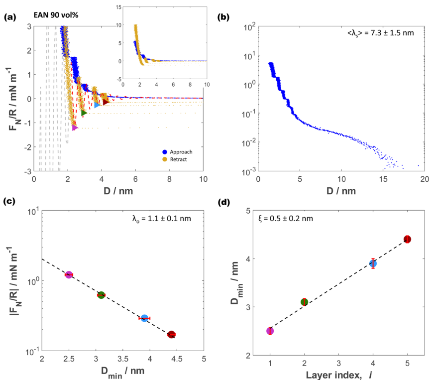
Fig. 3 Example measurements of the normalised force between mica sheets as a function of separation, D , across 90 vol% EAN. (a) Linear scale forces at D < 10 nm with retraction (gold) shown from each layer. Red dashed line shows the force fitted using eqn (1) and the parameters reported in Table 1. Inset shows the full magnitude of the force. (b) Log-linear representation of normal force displaying long-range decay with average decay length \langle \lambda_s \rangle = 7.3 \pm 1.5 nm. (c) The exponential decay envelope is calculated from the force minima, giving \lambda_o = 1.1 \pm 0.1 nm. (d) The distance separation between the minima gives the oscillation wavelength of the structural force, here \xi = 0.5 \pm 0.2 nm.
