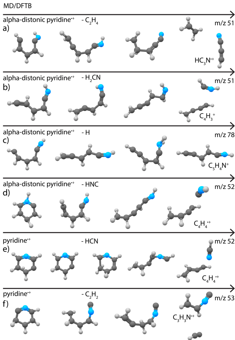
Fig. 7 Exemplary pathways for loss of (a) C 2 H 4 , (b) H 2 CN, (c) H and (d) HNC loss from alpha distic pyridine ++ and (e) HCN and (f) C 2 H 2 loss from canonical pyridine ++ as observed in the MD/DFTB simulations at 6.74 eV internal energy of the respective cation using Set1 parameters. The arrows indicate time.
