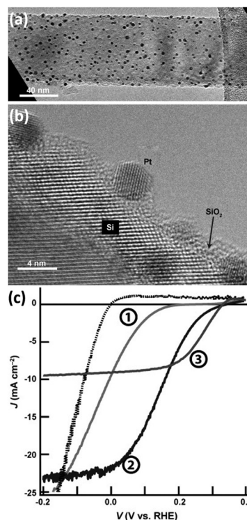
Fig. 10 (a) TEM and (b) HRTEM images of Pt nanoparticles modified Si nanowire, (c) PEC HER performance of naked Si nanowires (①), and Si nanowires modified with Pt nanoparticles by ELD (②) and ALD (③). Reproduced with permission from ref. 86, Copyright © 2013 Wiley-VCH Verlag GmbH & Co. KGaA, Weinheim.
