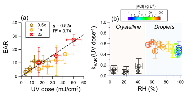
Fig. 3 (a) Endotoxin activity ratio as a function of UV dose, where 0.5x, 1x, and 2x represent the average UV irradiances of 35, 70, and 140 μW cm -2 , respectively. The bioaerosol was nebulized from water suspension. (b) Rate constant of the increase of endotoxin activity ratio as a function of RH. The [KCl] in the droplets (right region) was determined by hygroscopicity measurements at RH higher than efflorescence RH (Text S6, Fig. S5 and S6†). For an RH higher than 83%, which cannot be reached in the chamber, the results were obtained from illuminated aqueous suspension (Text S7 and Fig. S7†), and results of the illuminated crystalline particles were obtained from initially 2 g L -1 KCl droplets with 10 7 CFU mL -1 cells using a flow cell (black rhombuses, Text S8 and Fig. S5†) and a teflon chamber (black squares).
