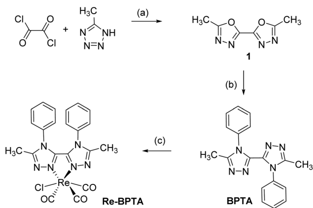
Scheme 1 Synthesis of the tricarbonylrhenium(i) complex Re-BPTA. (a) Xylenes, N 2 , 2 h, 120 °C, 69%; (b) Xylenes, aniline (3.6 eq.), p -TsOH.H 2 O (0.3 eq.), 18 h, 140 °C, 92%; (c) [ReCl(CO) 3 ] (1.3 eq.), butan-2-ol, 100 °C, 18 h, 73%.
