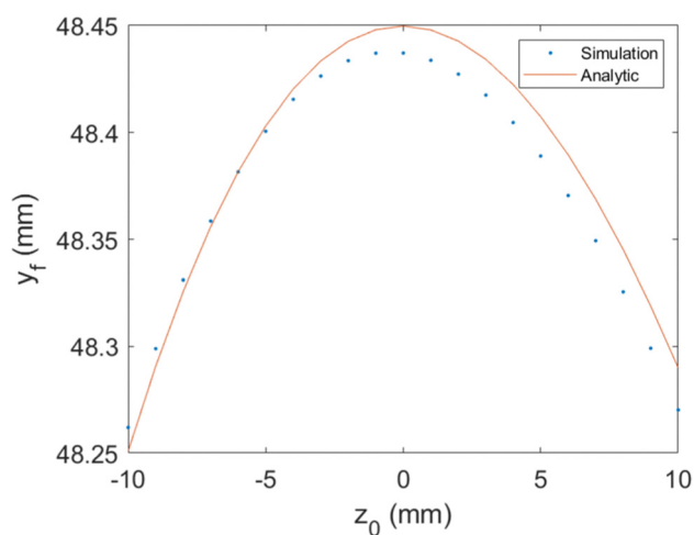
Fig. 6 Impact position y_f as a function of the source position z_0 , for \epsilon_{\text{max}} = 1.8 eV. We used an electron beam starting from the origin with velocity on the y axis only, which corresponds to a kinetic energy of 1 eV. We observe very small deviations (less than 0.041%) that practically can be neglected, since they are smaller than the detector's resolution.
