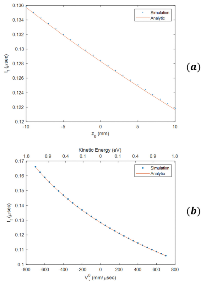
Fig. 5 (a) Time-of-flight for a beam of electrons starting from different positions along the \hat{z} axis between z_0 = -10 mm to z_0 = 10 mm, for x_0 = y_0 = 0 , and for \epsilon_{\text{max}} = 1.8 eV. (b) Time-of-flight for a beam of electrons starting from the origin with velocity on z axis only for \epsilon_{\text{max}} = 1.8 eV.
