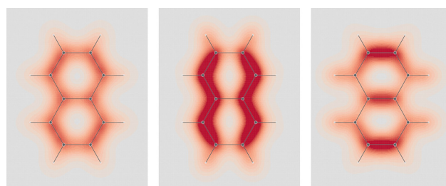
Fig. 3 EDPD of naphthalene over a plane located at 1 a.u. below the molecular plane. Left \mathcal{N}_{av} ; center and right in-plane components. See caption to Fig. 1 for other details.
