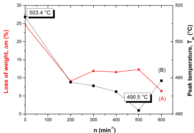
Fig. 9 The loss of weight \Delta m (A) and peak temperature T_m (B) of mechanically activated chalcopyrite \text{CuFeS}_2 vs. mill revolutions n .
