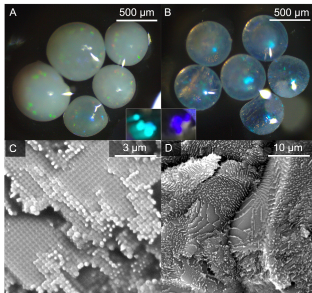
Fig. 2 Optical micrographs of (A) 370PC <math>C</math> CsPbBr 3 and (B) 190PC <math>C</math> CsPbCl 1.5 Br 1.5 microbead hybrids exposed to light from above in silicone oil with insets of hybrids illuminated with \lambda_{\text{ex}} = 365 nm. SEM of (C) 370PC <math>C</math> CsPbBr 3 and (D) 190PC <math>C</math> CsPbCl 1.5 Br 1.5 .
