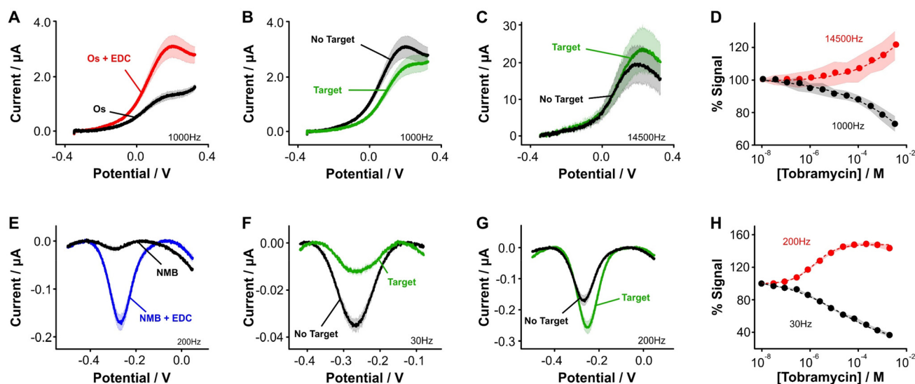
Fig. 3 Aptamer-bound [\text{Os}(\text{dmbpy})_2\text{Cl}(\text{ampy})]^+ supports E-AB sensing. (A) Using the carboxylic group at the terminal end of immobilized tobramycin aptamers and the free amine group in the Os complex, we successfully attached the complex to the DNA strands via EDC chemistry. (B and C) [\text{Os}(\text{dmbpy})_2\text{Cl}(\text{ampy})]^+ sensors signal output to target additions at \sim 1000 Hz and \sim 14\,500 Hz, respectively. These square wave frequencies were determined from the frequency maps shown in Fig. S5. † (D) Such signaling is used to build calibration curves where the normalized response changes monotonically with target concentration. The signaling is reversible under continuous voltammetric interrogation (Fig. S7, ESI † ). (E–G) Control NMB-modified sensors also display signal-OFF and signal-ON responses, albeit at lower frequencies: \sim 30 Hz and \sim 200 Hz, respectively. These square wave frequencies are the standard for interrogation of MB-based tobramycin sensors. 5 (H) NMB-modified sensors achieve larger signal gain and display better affinity for the same target (tobramycin). Solid lines/dots and shaded areas represent the average and standard deviation of 4 sensors.
