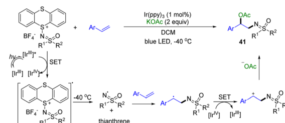
In 2020, Ritter reported a photocatalytic allylic C–H amination reaction of alkenes and iminothianthrene to prepare aliphatic allylamines (Scheme 40). 102 The proposed mechanism shows that the excited iridium photocatalyst was quenched by protonated iminothianthrene to generate an excited complex via energy transfer, which underwent further protonation to afford a cationic nitrogen radical intermediate and thianthrenium radical cation. The cationic nitrogen radical was added to alkenes regioselectively to afford an alkyl radical, which recombined with a thianthrenium radical cation to
