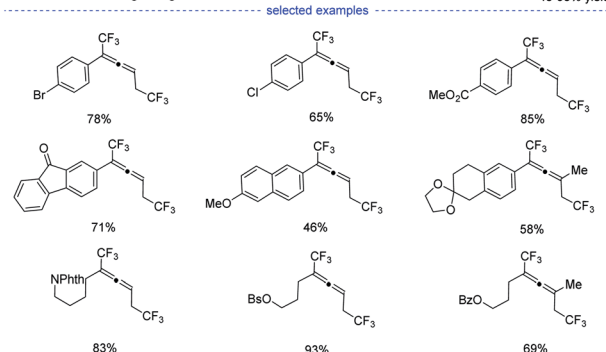
Scheme 10 Cu-catalyzed three-component 1,4-bis(tri-fluoromethylation) of 1,3-enynes.
