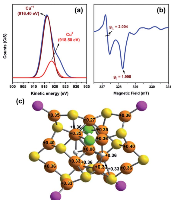
Fig. 5 (a) Deconvoluted \text{Cu LMM} Auger spectrum of the \text{Cu}_{18}\text{NC} , (b) EPR spectrum of the \text{Cu}_{18}\text{NC} , and (c) Bader charge analysis of the optimized \text{Cu}_{18}\text{NC} . Color legend: Cu, orange; S, yellow; P, magenta; Cl, green; H, white. For clarity, all phenyl and adamantane groups are omitted.
