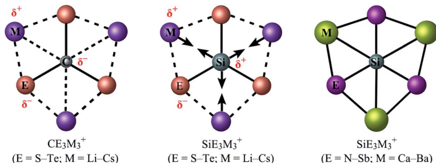
Fig. 1 The pictorial depiction of previously reported phC \text{CE}_3\text{M}_3^+ (E = S-Te; M = Li-Cs) clusters and the present \text{SiE}_3\text{M}_3^+ (E = S-Te and N-Sb; M = Li-Cs and Ca-Ba) clusters. Herein the solid and dashed lines represent covalent and ionic bonding, respectively. The opposite double arrows illustrate electrostatic repulsion.
