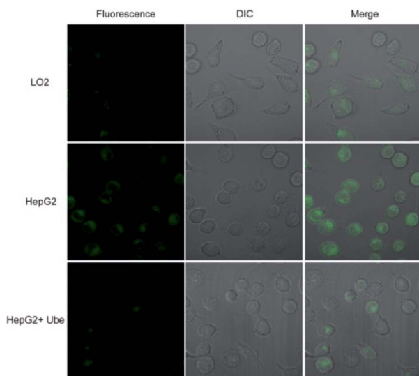
Fig. 6 Confocal fluorescence (Flu) imaging of LO2 and HepG2 cells treated with probe 1 (10 \mu M) or probe 1 plus Ube (40 \mu M) for 1 h. The fluorescence was acquired at 500–650 nm upon excitation at 405 nm.
