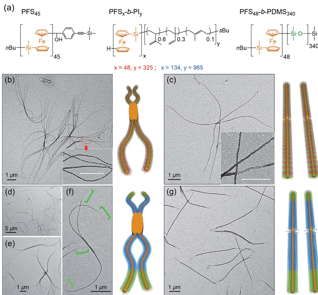
Fig. 6 (a) Chemical structures of the PFS homopolymer and the three block polymers employed. In the drawings to the right of each set of TEM images we use orange to indicate the location of PFS, red/blue to indicate the location of the PI corona chains, and green to indicate the location of the PDMS corona chains. (b and c): TEM images of the micelles formed by \text{PFS}_{45}/(\text{PFS}_{48}\text{-}b\text{-PI}_{325} + \text{PFS}_{48}\text{-}b\text{-PDMS}_{340}) (0.5 w/w%, BCP mass ratio 2 : 3). The mixture was heated at 90 °C for 30 min. (b) Branched structures formed upon rapid cooling; (c) linear structures formed upon slow cooling. (d–f): TEM images of the micelles formed by \text{PFS}_{45}/(\text{PFS}_{134}\text{-}b\text{-PI}_{965} + \text{PFS}_{48}\text{-}b\text{-PDMS}_{340}) (0.5 w/w%, BCP mass ratio 5 : 1). The mixture was heated at 100 °C for 30 min. Branched block comicelle structures formed upon rapid cooling. (g) Same sample as in (d–f) but linear block comicelle structures formed upon slow cooling. The PI bloc was stained with Karstedt's catalyst to show the patchy structure of the corona in (b and c), and the block comicelle structure in (d–g).
