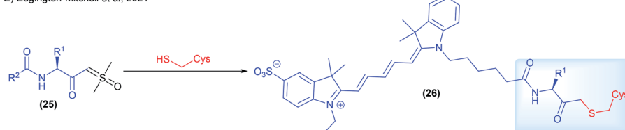
Scheme 5 Industrial research and applications relating to sulfoxonium ylides in X–H insertion reactions.
