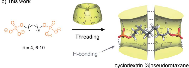
Fig. 1 (a) Previous work on compression of alkyl chains by self-assembled capsules or boxes. (b) Alkyl diphosphate axles used in this study and corresponding CD [3]pseudorotaxane with potential compression resulting from hydrogen bonding and hydrophobic interactions between the threaded axle and head to head CDs.
