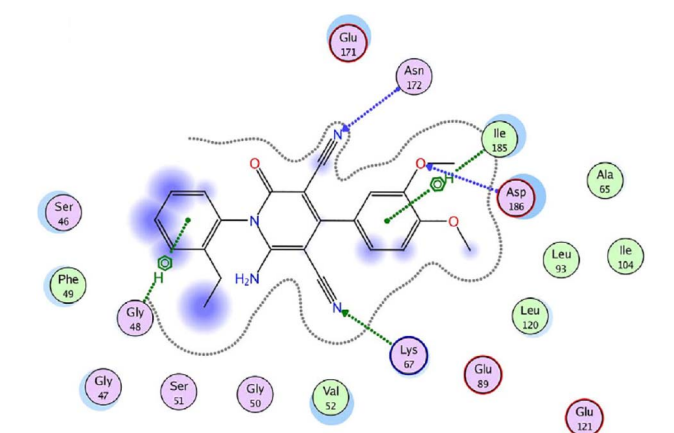
Fig. 4 2D interactions of compound 25g with Pim-1 kinase (PDB ID code: 2OBI). Reproduced with permission from ref. 53. Copyright John Wiley & Sons Inc., 2022.
