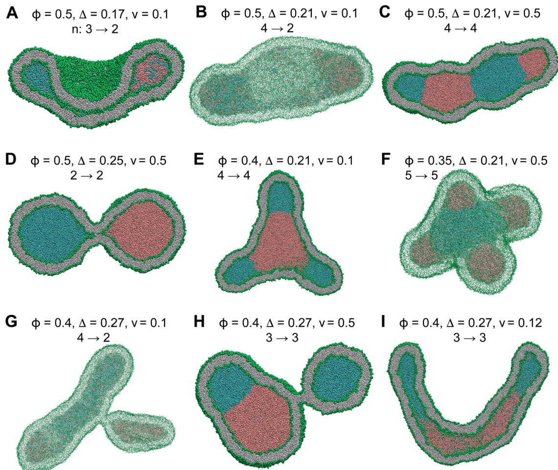
Fig. 3 Morphological transformations of stable and meta-stable compartmentalized vesicles with different values of \phi , v , and \Delta for a fixed p = 2 , corresponding to \lambda = -2.6 k_B T/d and \Sigma_{\alpha\beta} = 1.88 k_B T/d^2 . (A) A cup-shaped vesicle at small \Delta = 0.17 . (B) A meta-stable sheet structure. (C) A meta-stable long-lived tubular vesicle. (D) A stable dumbbell with circular neck at high \Delta = 0.25 . (E) A meta-stable branched tubule. (F) A meta-stable five-compartment vesicle. (G) A meta-stable branched tubule. (H) A meta-stable three-compartment vesicle. (I) A meta-stable long tubule at high \Delta = 0.27 . The number n of the initial and final compartments of the vesicles are shown by arrows above each vesicle. Morphological transitions of multi-compartment vesicles.
