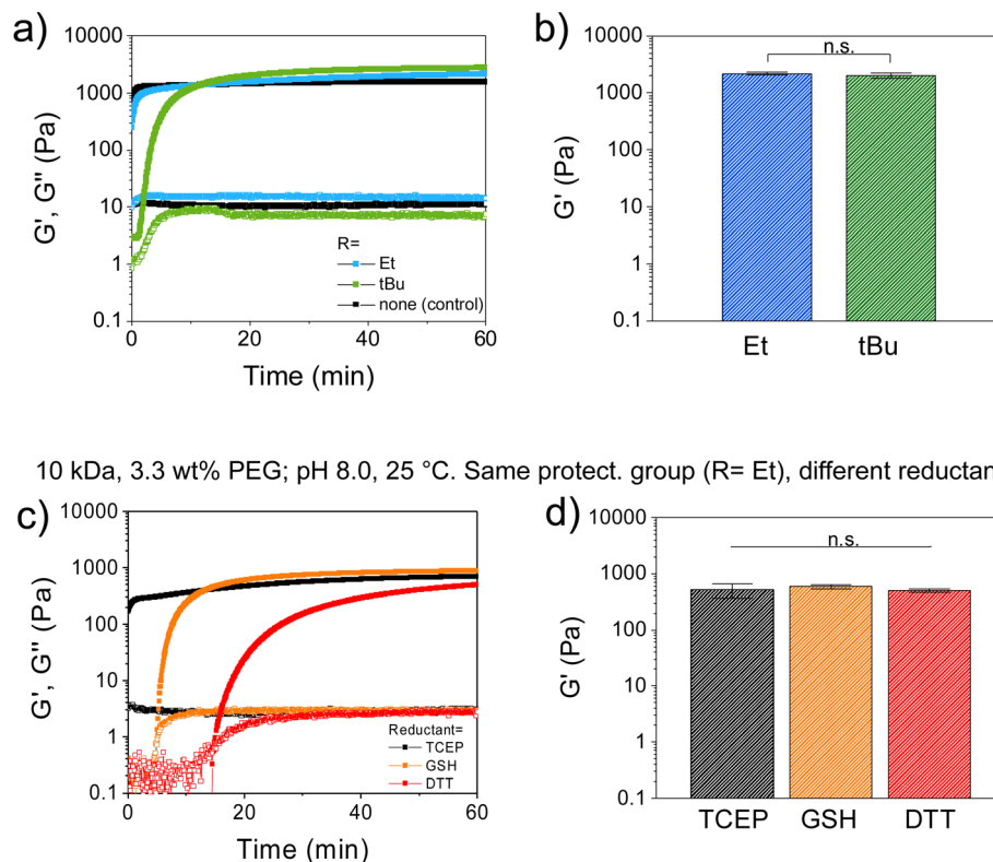
Fig. 2 Study of gelation kinetics and mechanical strength of redox-triggered hydrogels by shear oscillatory rheometry, at varying Cys protecting group and reductant type. Shear storage ( G' ) and loss ( G'' ) moduli were followed as a function of time and denoted as closed and open symbols, respectively. (a and b) Effect of different Cys-protecting groups of PEG-Cys(SR) precursor, on the gelation of CBT-Cys(SR) gels under constant reductant type (TCEP), before (a) and after (b) swelling. A CBT-Cys gel, prepared from unprotected PEG-Cys is shown as control. (c and d) Effect of reductant type (TCEP, GSH or DTT) on the gelation of CBT-Cys(StBu) gels, before (c) and after (d) swelling (i.e., at constant protecting group). Gel composition: (a and b) 20 kDa PEGs, 5 wt% polymer content, in HEPES buffer, at (1 : 1) reductant : Cys(SR) molar ratio, T = 25 °C. (c and d) 10 kDa PEGs, 3.3 wt% polymer content, in HEPES, at (1 : 1) reductant : Cys(StBu) molar ratio, T = 25 °C. The reductant used is indicated in each case. In all cases, data are plotted as mean \pm SD, n = 3 . In (b) & (d), statistical significance was analyzed by ANOVA followed by the post hoc Tukey test ( *p < 0.05 set for statistical significance level; n.s. = not significant).
