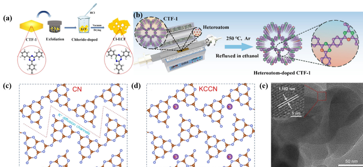
Fig. 11 (a) Schematic diagram of the preparation for Cl-ECF photocatalysts. Reproduced from ref. 128 with permission from Elsevier, Copyright 2020. (b) Schematic illustration of the synthetic process of HA-CTF-1. Reproduced from ref. 129 with permission from the American Chemical Society, Copyright 2022. Proposed molecular structure for (c) CN and (d) KCCN. Reproduced from ref. 132 with permission from the American Chemical Society, Copyright 2021. (e) HRTEM image of KCCN. Reproduced from ref. 132 with permission from the American Chemical Society, Copyright 2021.
