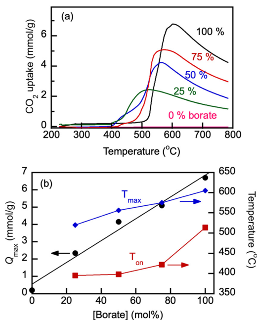
Fig. 7 \text{CO}_2 uptake ( Q , \text{mmol g}^{-1} ) by molten borate/carbonate blends under the 60\text{ mL min}^{-1} flow of 100% \text{CO}_2 at a heating rate of 5\text{ }^\circ\text{C min}^{-1} (a) and dependencies of the maximum \text{CO}_2 loading ( Q_{\text{max}} ), temperature of the onset of the loading increase ( T_{\text{on}} ), and the temperature of the maximum \text{CO}_2 loading ( T_{\text{max}} ) on nominal content of Li, Na borate, in the borate/carbonate blends (b). In the TGA experiments, the blends were first purged of water and \text{CO}_2 by exposing them to \text{N}_2 flow and ramping the temperature to 600 ^\circ\text{C} at 5\text{ }^\circ\text{C min}^{-1} and then allowing to equilibrate, also under \text{N}_2 flow, at 200 ^\circ\text{C} for 1 h. The \text{CO}_2 loading was calculated as a sample weight fraction gained on the exposure to the \text{CO}_2 flow, normalized by the molar mass of \text{CO}_2 ( 44.01\text{ g mol}^{-1} ). Numbers indicate nominal initial content of borate (mol%) in the blends.
