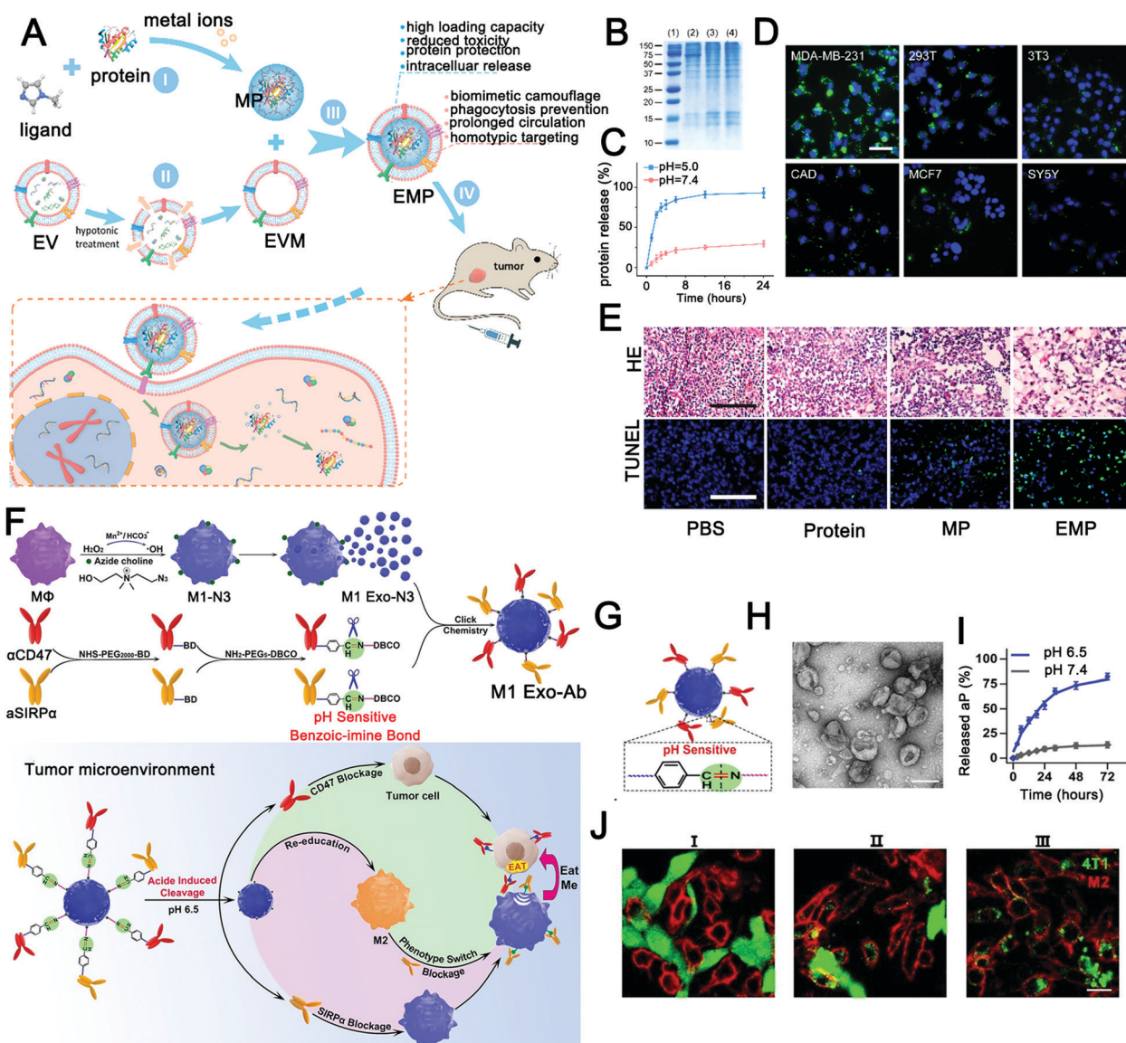
Fig. 2 Engineered extracellular vesicles for pH-responsive delivery of drugs. (A) Schematic diagram of homologous targeting protein intracellular delivery with pH-responsive biomimetic EMP NPs. (B–E) Cell and tissue level experiments verified the homologous targeting, pH response, and antitumor effect of biomimetic EMP nanoparticles. (Reprinted with permission from ref. 213, Copyright 2018 American Chemical Society.) (F and G) Schematic of the construction of pH-responsive immunotherapeutic exosomes (M1 Exo-Ab) and the synergistic anticancer effect of M1 Exo-Ab. (H–J) The morphology, pH response, and antitumor effect of M1 Exo-Ab were verified in vitro . (Reprinted with permission from ref. 43, Copyright 2020 Wiley-VCH Verlag GmbH & Co. KGaA, Weinheim.)
