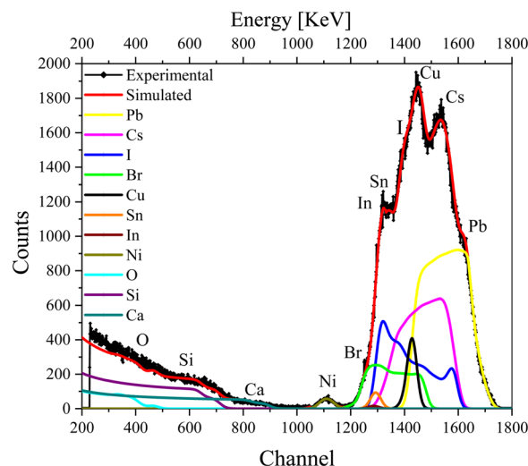
Fig. 4 RBS spectrum of the complete device excited from the Cu contact side, with simulation and deconvolution of the elemental spectra for glass/ITO/NiO x /CsPbI 2 Br/C 60 /Cu.
