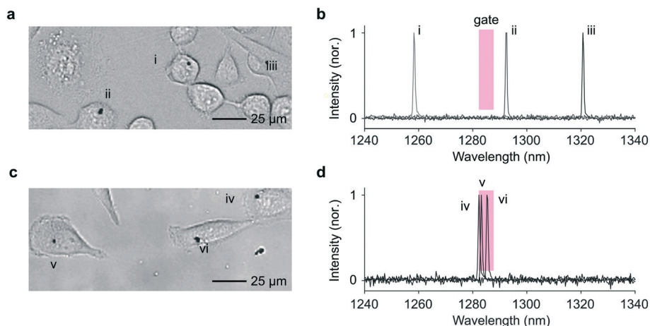
Fig. 6 Band-pass sorting. a, A bright-field image of replated cells collected from the (–) outlet. b, The LP laser emissions from the LPs labelled i, ii and iii. c and d, Image and emission spectra of cells collected from the (+) outlet, showing three LPs (iv–vi).
