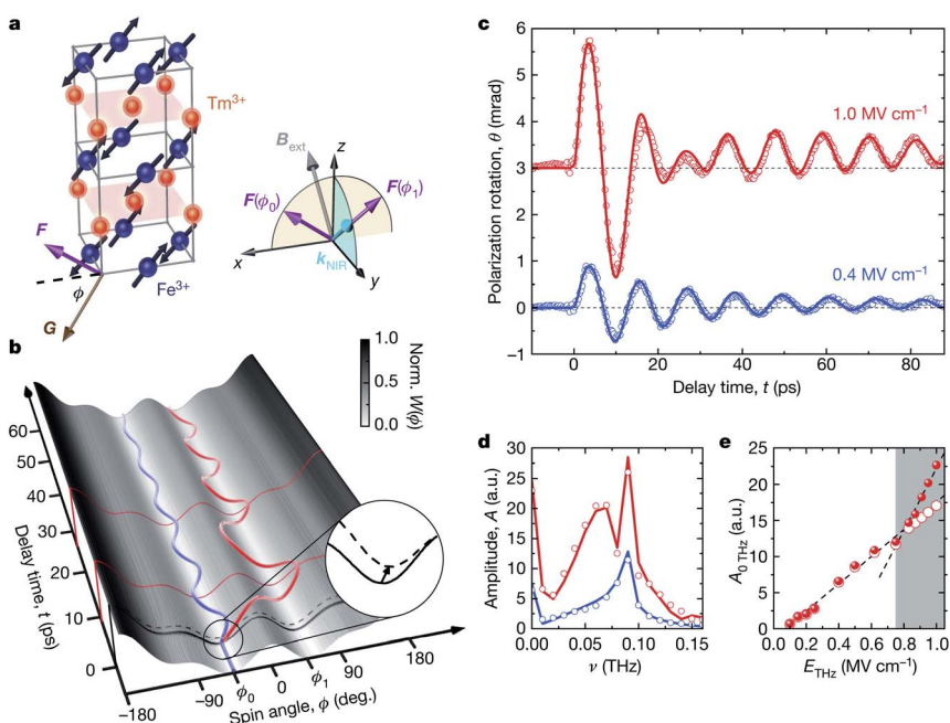
Fig. 3 THz-driven switching in the canted antiferromagnet \text{TmFeO}_3 . (a) The structure of \text{TmFeO}_3 , showing the sublattice spin orientations and the direction of the net magnetic moment. (b) A sketch of the magnetic potential energy and spin dynamics for low (blue) and high (red) field excitations. (c) Measured dynamics of the Faraday rotation angle, an experimental measure of the spin angle orientation. (d) Amplitude of the Fourier transform of the data in panel c. (e) Simulated behavior of the long-lived offset in the Faraday rotation as a function of the excitation level for two alignments of the near-infrared probe (red circles and red spheres). The difference at high fields is a consequence of the metastable transfer of spins over the potential energy barrier. Reprinted with permission from Nature 65 [Schlauderer et al. , Temporal and spectral fingerprints of ultrafast all-coherent spin switching]. Copyright 2019 Springer Nature.
