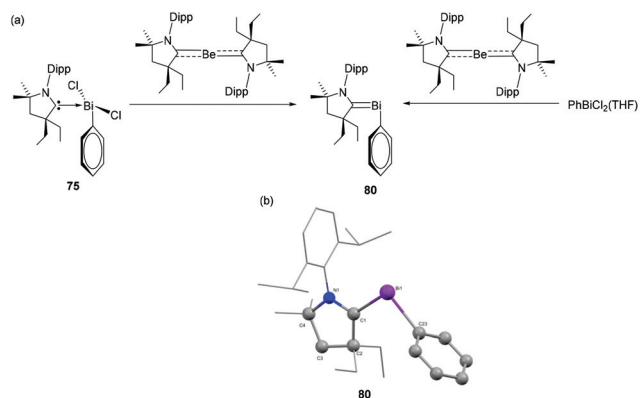
Fig. 26 (a) Synthesis of carbene-stabilized bismuthinidene compound 80 , (b) solid-state structure of 80 .
