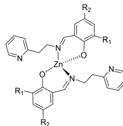
Scheme 2 Structures of the homoleptic Zn(II) complexes 1 – 6 .
