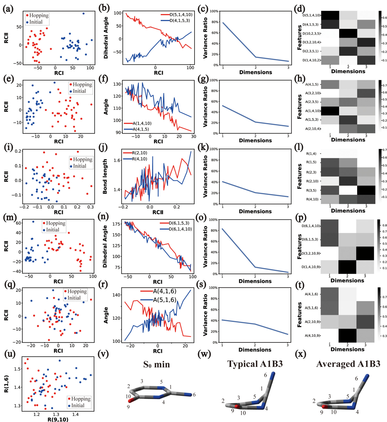
Fig. 6 The analysis results of Cluster A1B3 . (a)–(d), (e)–(h), (i)–(l), (m)–(p) and (q)–(t) The PCA results of D_{ring} , A_{ring} , R_{ring} , D_{eg} and A_{eg} , respectively. (u) The distributions of R(9,10) and R(1,6) . (v)–(x) Represent the S_0 minimum, the typical structures and the averaged structures, respectively.
