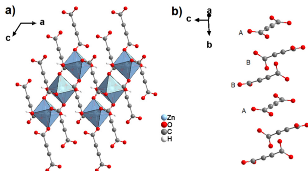
Fig. 46 Sections of the crystal structures of [Zn(ADC)(H 2 O) 2 ] (a) and [Ce 2 (ADC) 3 (H 2 O) 6 ]. 2 H 2 O (b), disclosing short C≡C...C≡C contacts between neighbouring ADC ligands. The coordination sphere of Ce 3+ is omitted in (b) for clarity. Graphics redrawn from the cif file (CSD-Refcode DAYMAS and KAPHAL). 54,84
