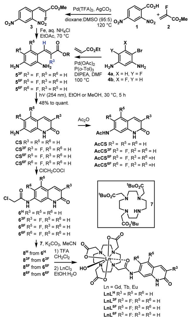
Scheme 1 Preparation of CS F , AcCS , AcCS F , and LnL F .
