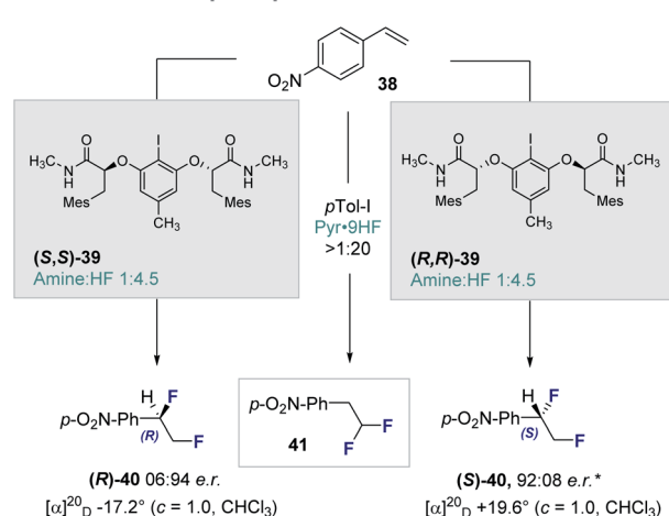
Fig. 9 The enantioselective, catalytic vicinal difluorination of electron deficient styrenes. * 98 : 2 e.r. after recrystallisation from \text{CH}_2\text{Cl}_2/n -pentane.
