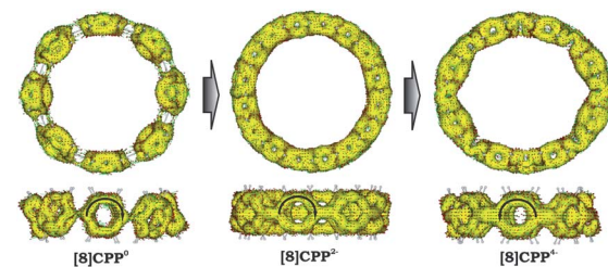
Fig. 10 \pi -Contribution to the ACID isosurface for 1^0 , 1^{2-} , and 1^{4-} (PBE0/cc-pVTZ). Current density vectors are plotted onto the ACID isosurface to indicate diatropic and paratropic ring currents.
