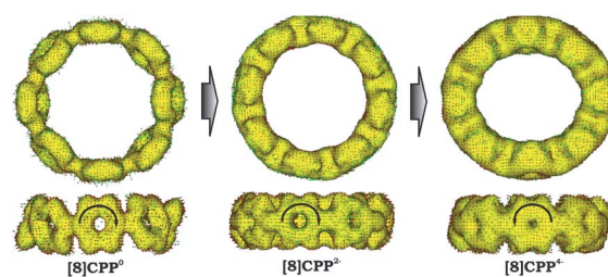
Fig. 9 Full ACID isosurfaces for 1^0 , 1^{2-} , and 1^{4-} (PBE0/cc-pVTZ). Current density vectors are plotted onto the ACID isosurface to indicate diatropic and paratropic ring currents.
