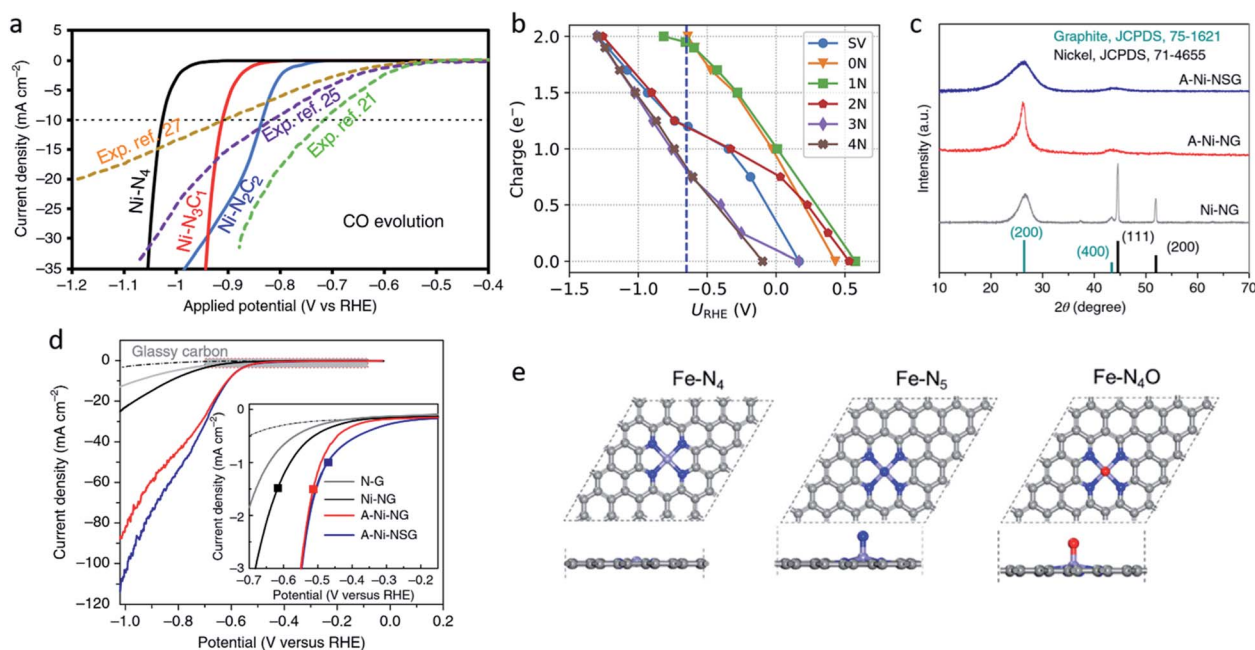
Fig. 3 (a) Calculated j_{CO} values in the CO 2 RR on Ni-N 2 C 2 , Ni-N 3 C 1 , and Ni-N 4 . Reproduced from ref. 75 with permission from Springer Nature, copyright 2020. (b) Charge capacities of different sites under different potentials for *COOH. Reproduced from ref. 77 with permission from the American Chemical Society, copyright 2020. (c) XRD patterns and (d) LSV curves for A-Ni-NSG, A-Ni-NG, and Ni-NG. Reproduced from ref. 26 with permission from Springer Nature, copyright 2018. (e) Top views and side views of the Fe-N 4 , Fe-N 5 and Fe-N 4 O sites. Reproduced from ref. 78 with permission from Elsevier, copyright 2020.
