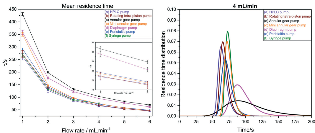
Fig. 17 Left: Mean hydrodynamic residence times as derived from RTD measurements of the FlowNMR apparatus shown in Fig. 12 with pumps (a–f). Right: Comparison of RTD profiles of pumps (a–f) at 4 \text{mL}\cdot\text{min}^{-1} .
