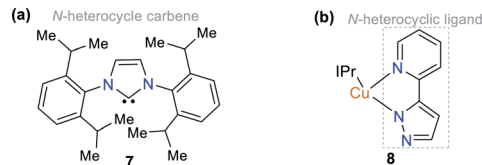
Fig. 3 Structure of (a) ligand IPr 7 and (b) Cu(i) complex 8 .
