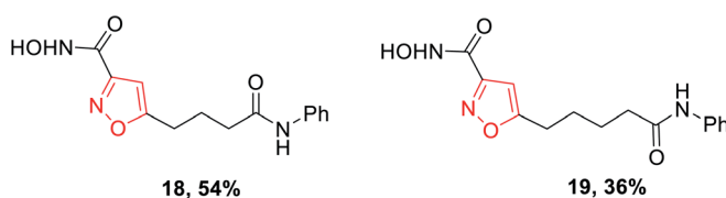
Scheme 3 Microwave-assisted metal-free routes to 3,5-disubstituted isoxazoles.
