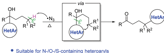
Scheme 1 Radical-mediated heteroarylation of unactivated C(sp 3 )-H bonds by means of functional group migration.
