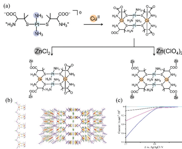
Fig. 4 \text{Pt}^{\text{II}}\text{--Cu}^{\text{II}}\text{--Zn}^{\text{II}} trimetallic coordination polymers as \text{O}_2 evolution electrocatalysts: (a) synthesis schemes, (b) packing structures of (left) a Cl salt and (right) a \text{ClO}_4 salt, and (c) LSV curves in \text{CH}_3\text{CN--H}_2\text{O} containing 0.1 M \text{KPF}_6 with a sample-modified glassy carbon electrode at a scan rate of 0.01 \text{ V s}^{-1} . Adapted from ref. 80 with permission from The Royal Society of Chemistry.
