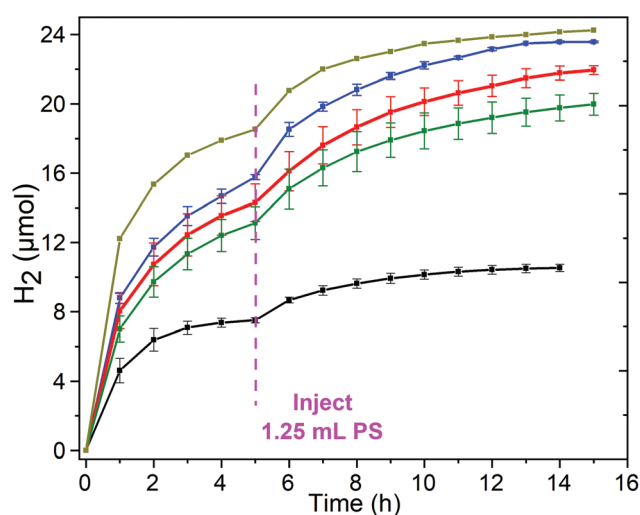
Fig. 6 Hydrogen evolution-time profile for copper complexes 1 – 3 in DMF ( C_{\text{cat}} = 5 \mu\text{M} ), with a fresh 1.25 \text{ mL} aliquot of PS solution ( 0.2 \text{ mM} ) added after 5 \text{ h} , (blue) 1 [\text{Cu}^{\text{II}}\text{L}^{\text{Et}}]\text{BF}_4 , (red) 3 [\text{Cu}^{\text{II}}\text{L}^{\text{EtPy2}}]\text{BF}_4 and (green) 2 [\text{Cu}^{\text{II}}\text{L}^{\text{Et-MePy}}]\text{BF}_4 as well as for the 'blank' run with 0.2 \text{ mM} [\text{Ru}(\text{bpy})_3](\text{PF}_6)_2 (black) and the control experiment of \text{Cu}(\text{BF}_4)_2 salt (dark yellow). Conditions: Irradiation with a blue LED ( \lambda = 445 \text{ nm} , 88 \text{ mW cm}^{-2} ) at 20^\circ\text{C} , with 1.0 \text{ M} TEOA, 0.2 \text{ mM} [\text{Ru}(\text{bpy})_3](\text{PF}_6)_2 and 0.1 \text{ M} \text{HBF}_4/0.53 \text{ M} \text{H}_2\text{O} . Error bars show the standard deviation from the mean, calculated from two separate runs (Table 3 and Fig. S18–S21†).
