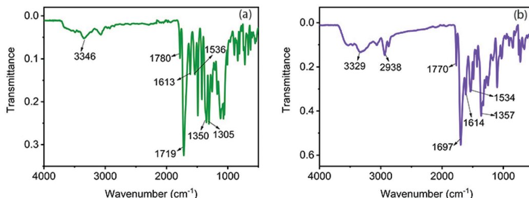
Fig. 1 FTIR spectra of the cPI films: (a) AMDA/TFDB; (b) AMDA/t-CHDA.
