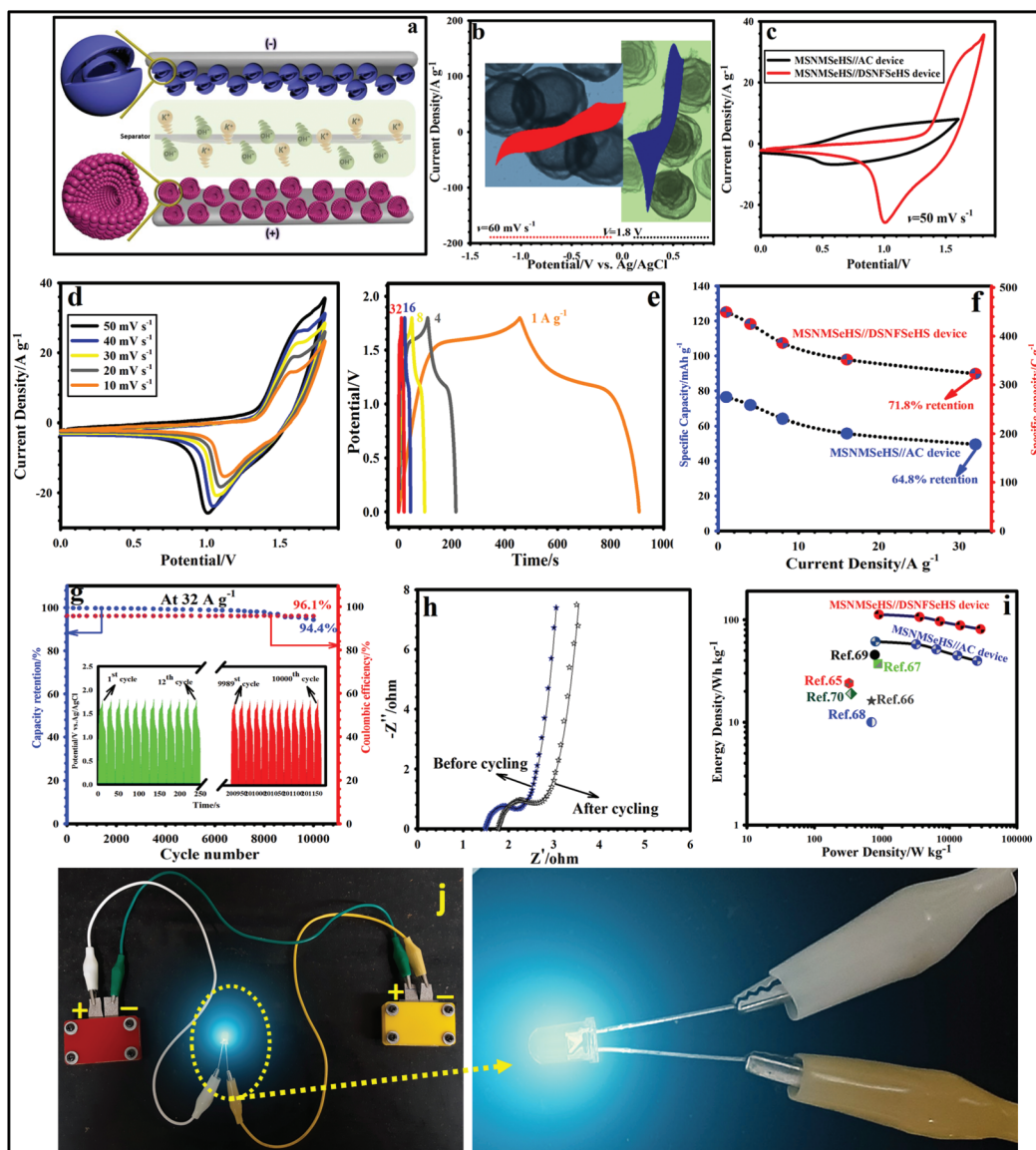
Fig. 6 (a) Schematic showing the MSNMeSeHS||DSNFSeHS device. (b) CV plots of the MSNMeSeHS (cathode) and DSNFSeHS (anode) electrodes at a scan rate of 60 \text{ mV s}^{-1} . (c) CV curves of the MSNMeSeHS||DSNFSeHS and MSNMeSeHS||AC devices at 50 \text{ mV s}^{-1} . (d) CV plots of the MSNMeSeHS||DSNFSeHS device at various sweep rates. (e) GCD profiles of the MSNMeSeHS||DSNFSeHS device at various current densities. (f) Rate capability of the MSNMeSeHS||DSNFSeHS and MSNMeSeHS||AC devices. (g) Cyclability and coulombic efficiency of the MSNMeSeHS||DSNFSeHS device. (h) Nyquist plots of the MSNMeSeHS||DSNFSeHS device before and after cycling. (i) The comparison of the Ragone plot of the MSNMeSeHS||DSNFSeHS device with some reports. (j) Photograph of the blue LED with two devices connected in series.
